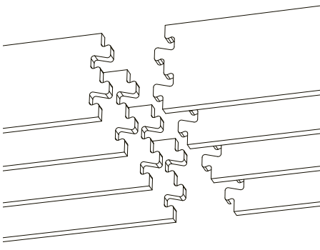
DOVETAIL JOINT
